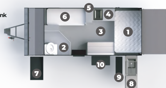
FLOOR PLAN SHOWN: OPTION ONE
